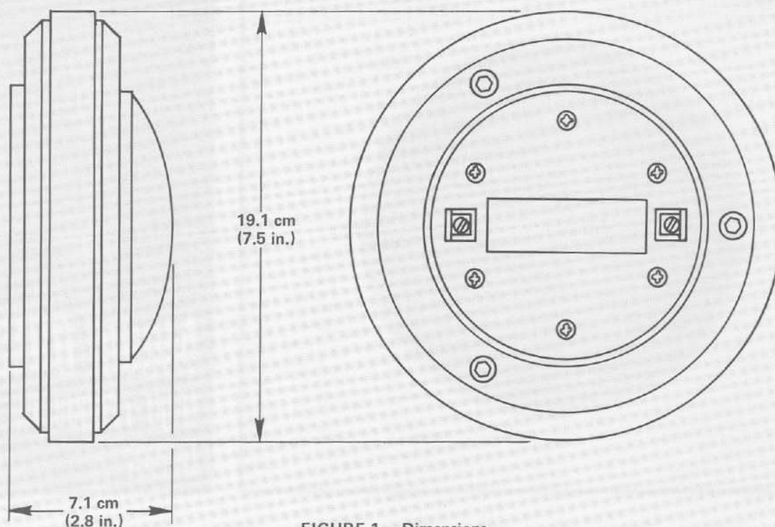
FIGURE 1 — Dimensions
